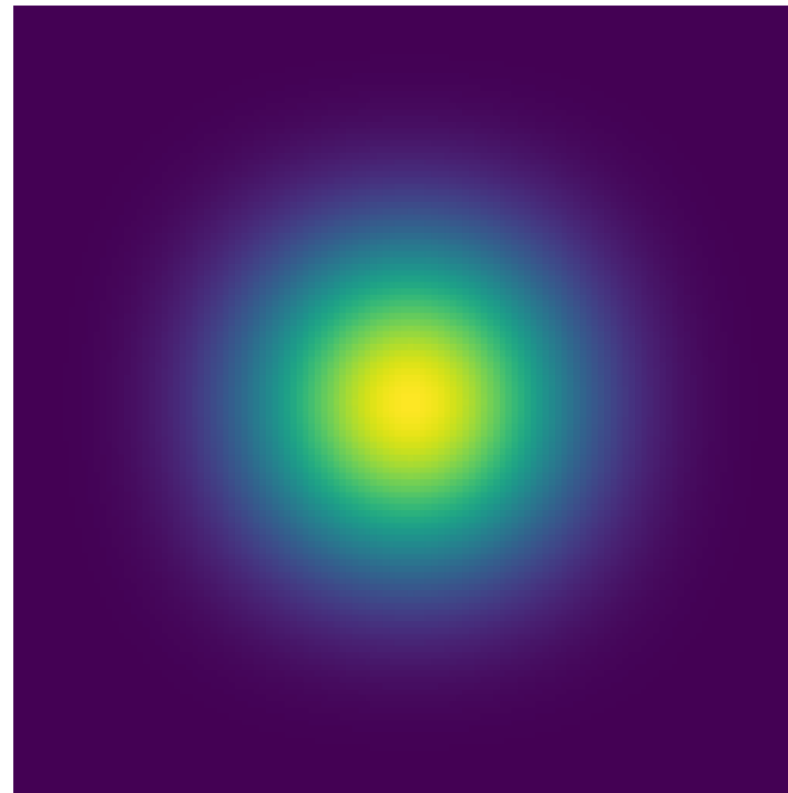
Blackman-Harris
