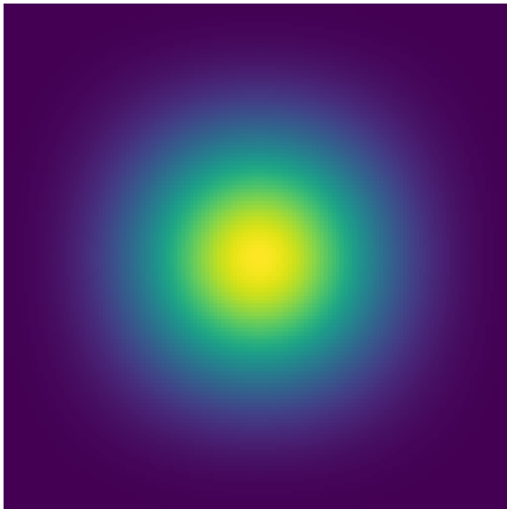
Blackman
